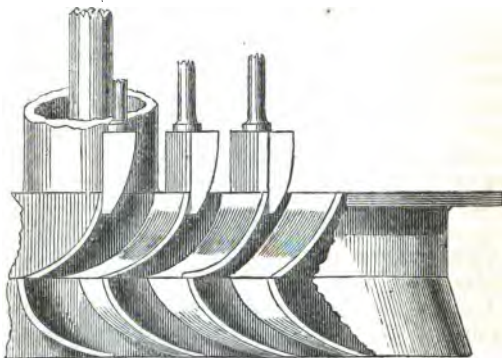
SECTIONAL ELEVATION, broken to show the form of the Guide Curves with three of the Sluces; also the form of the Buckets in the wheel below.
